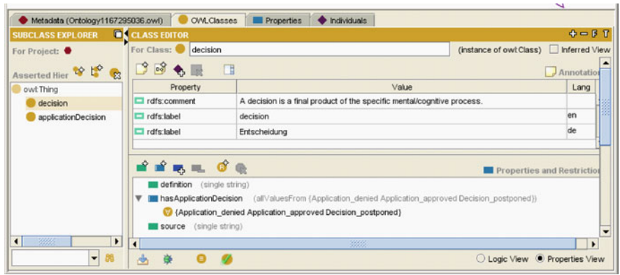
Fig. 19.10 Value restriction modelled in Protégé
